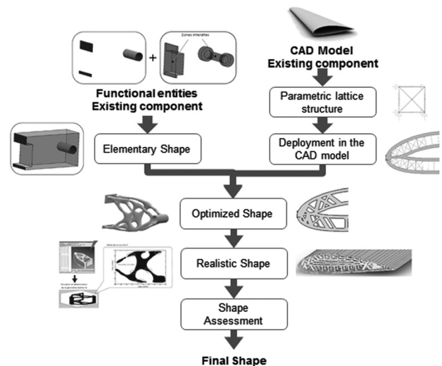
Fig. 3 Workflow of C-DFAM, adapted from Refs. [64] and [56]
