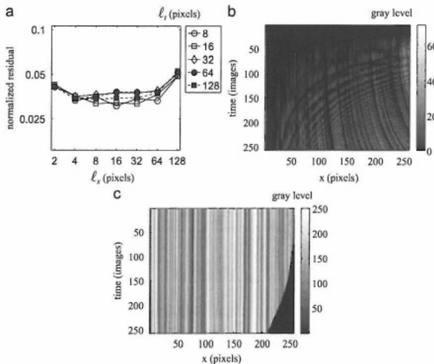
Fig. 8. Normalized mean gray level residual as a function of element size for a parabolic prescribed velocity (a). Residual map between the measured (with 32 × 32-pixel elements) and the prescribed trajectories (b). Corrected map with the measured displacement field for a 32 × 32 pixel element (c).
