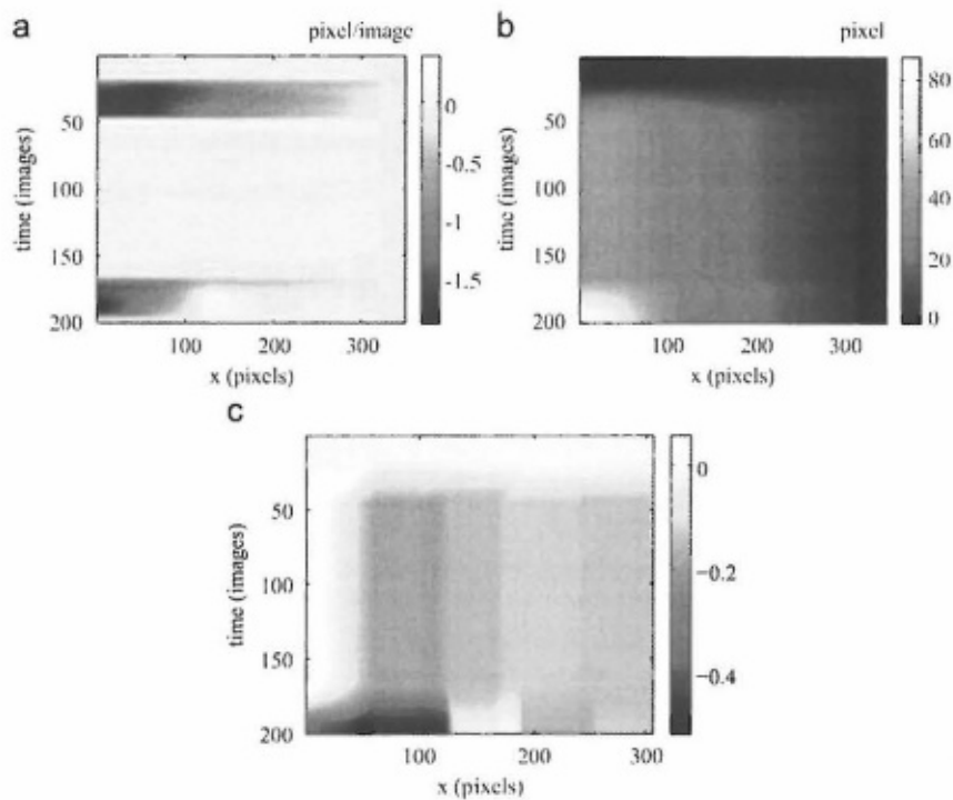
Fig. 12. Velocity (a), displacement (b) and engineering strain (c) maps for the studied test.
