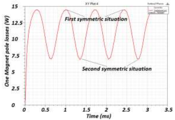
(d): Transient 2D finite elements calculation of magnet losses
