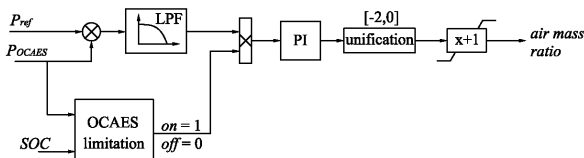
Fig. 8 Control scheme for OCAES
