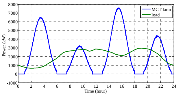
Fig. 2 Power curve of the studied MCT farm and load curve for a typical island in one day
