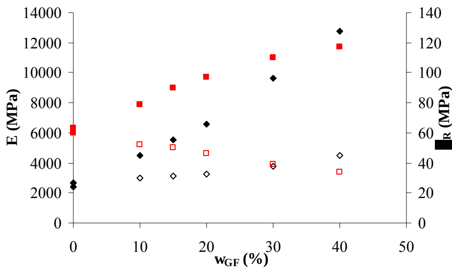
Figure 9. Young' modulus (◇,◆) and stress at break (■,□) for POM reinforced with glass beads (open symbols) and glass fibers (closed symbols) [98].
