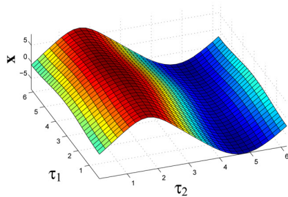
(c) Response at the resonance C ( \omega_1 = 4.582 , \|\tilde{\mathbf{x}}\| = 7.706 )
