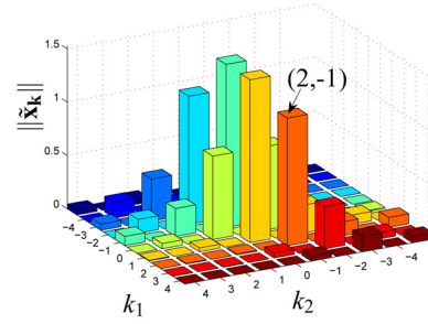
(a) Response at the resonance A ( \omega_1 = 1.678 , \|\tilde{\mathbf{x}}\| = 4.343 )
