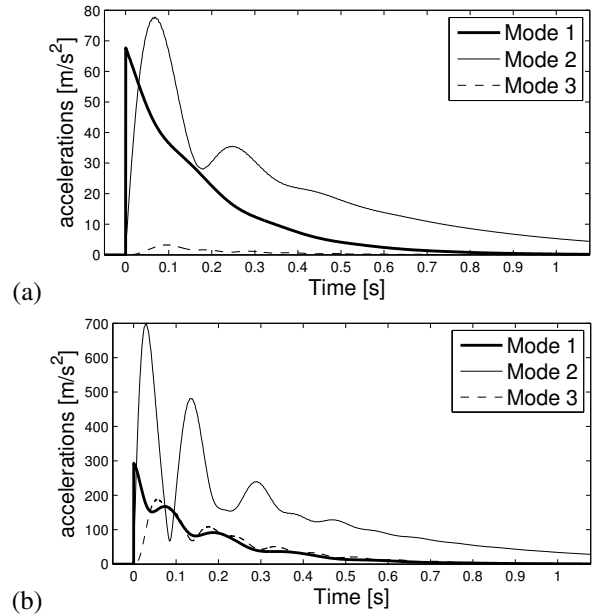
Figure 8. 1:2:4 internal resonance model in free oscillations simulation. Initial conditions in displacement: (a) w_0 = 0.15 mm, (b) w_0 = 0.65 mm.
