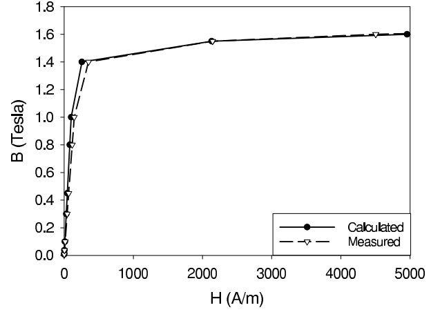
Fig. 3. Anhysteretic curve for the stator
