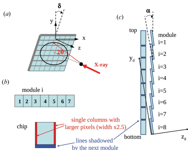
Figure 1 Schematic view of the geometry of the XPAD3.1 detector. (a) Experimental geometry with the tilt angle \delta between the average surface of the detector and the vertical direction y . 2\theta is the Bragg angle. (b) Description of a single module containing seven chips. (c) Side view of the detector showing the tiling of the modules with the tiling angle \alpha .
