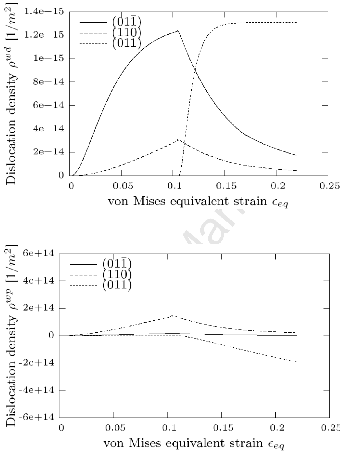
Fig. 10. Evolution of the intensity and polarity of the dislocation sheets in a crystal with initial orientation (32.9, 55.9, 137.4°) during the cross test described in Fig. 9.
