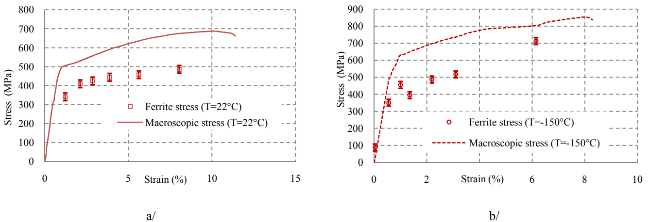
Fig. 4: Stress evolution in ferrite phase, 16MND5 steel - a/ T=22°C - b/ T=-150°C
