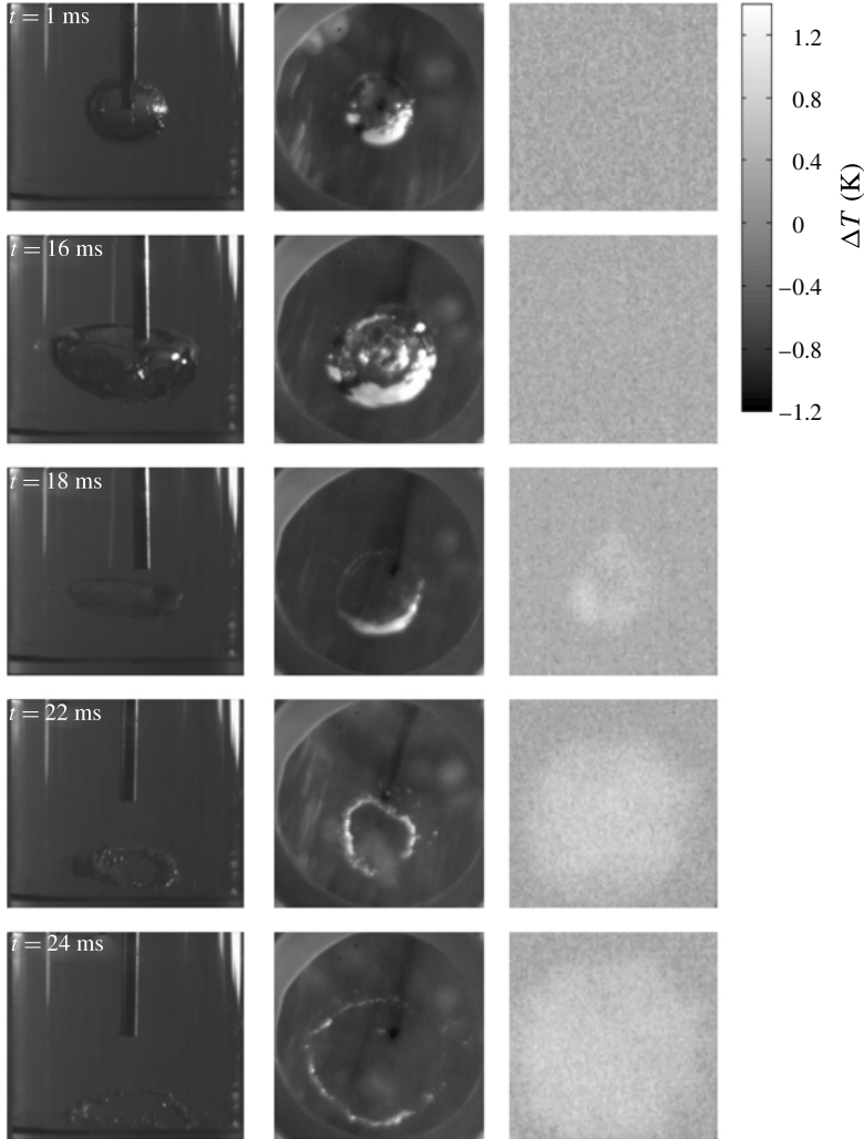
FIGURE 6. (Colour online) Evolutions of the bubble shape and temperature field for the case \chi = 1.3 .
