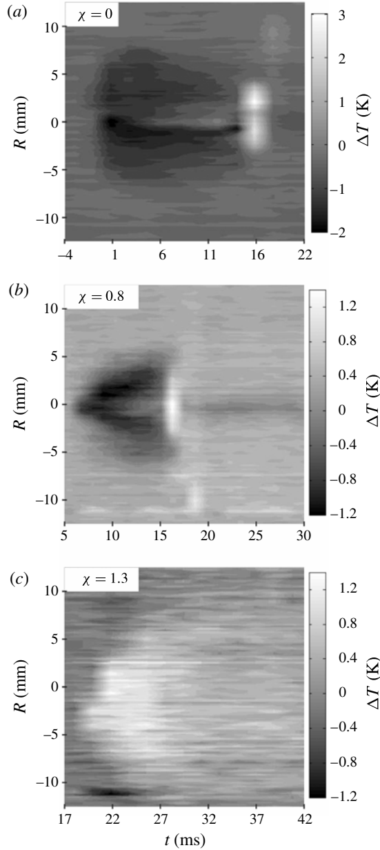
FIGURE 7. (Colour online) Temperature variations over time through vertical cross-sections of the bubble for non-dimensional standoff distances (a) \chi = 0 (for t = -4 to 22 ms), (b) \chi = 0.8 (for t = 5 to 30 ms) and (c) \chi = 1.3 (for t = 17 to 42 ms). Bubble growth begins at t = 0 .
