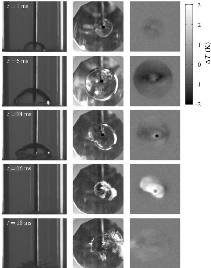
FIGURE 4. (Colour online) Evolutions of the bubble shape and temperature field for the case \chi = 0 .
