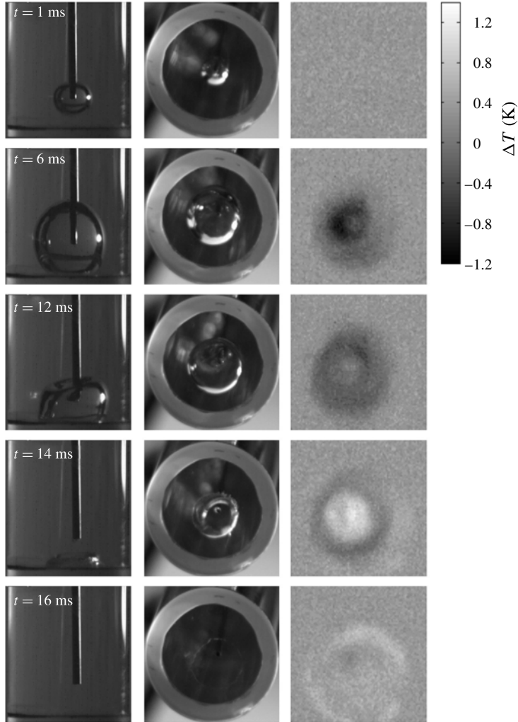
FIGURE 5. (Colour online) Evolutions of the bubble shape and temperature field for the case \chi = 0.8 .
