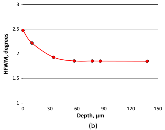
Fig. 11. (a) In-depth profile of initial surface residual stresses and (b) its corresponding profile of Full-width at Half maximum (FWHM) of the X-ray diffraction peaks measured in a virgin cylindrical specimen.
