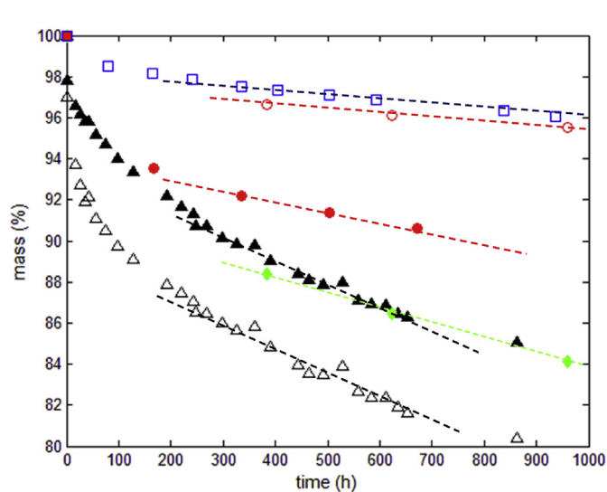
Fig. 3. Typical mass loss curves of UP for 200 \mu\text{m} ( \blacktriangle , \triangle ), 1 mm filled ( \blacklozenge , \circ ), 2 mm ( \bullet , \circ ), 5 mm ( \square ) aged under air at 160 °C. Open and closed symbols correspond respectively to unfilled and filled materials. The dashed lines correspond to the "stationary regime" where the mass loss rates were determined (see text).
