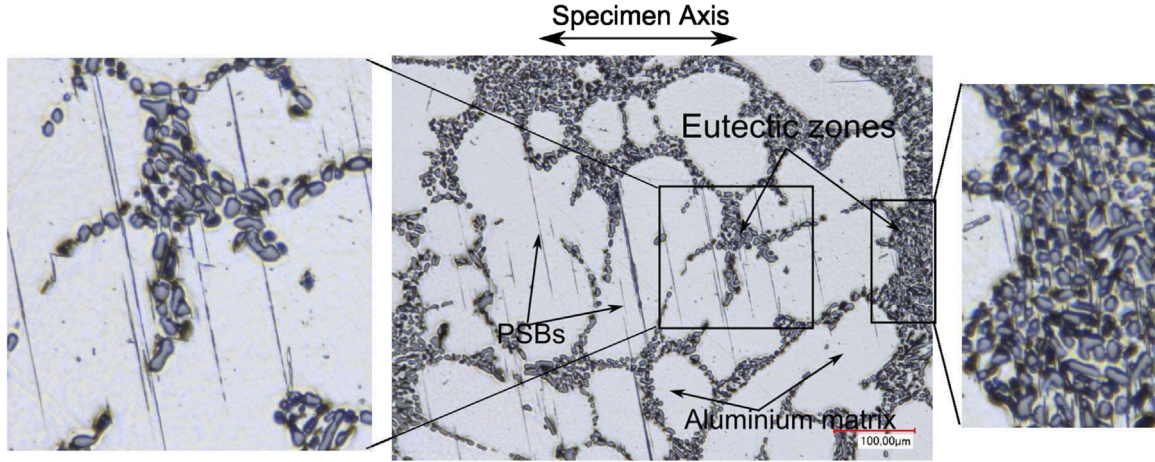
Fig. 19. PSB observed on an alloy C specimen subject to pure torsion with \tau_q = 80 MPa at N = 2.2 \times 10^6 cycles.
