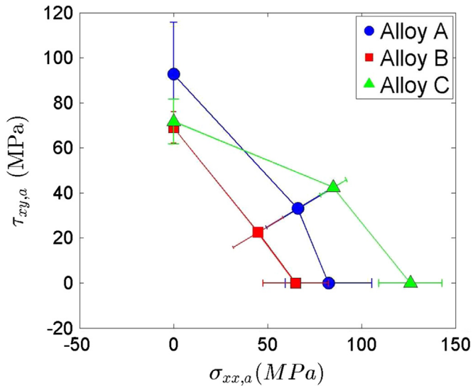
Fig. 9. \tau_{xy,\alpha} - \sigma_{xx,\alpha} diagram of three studied alloys.
