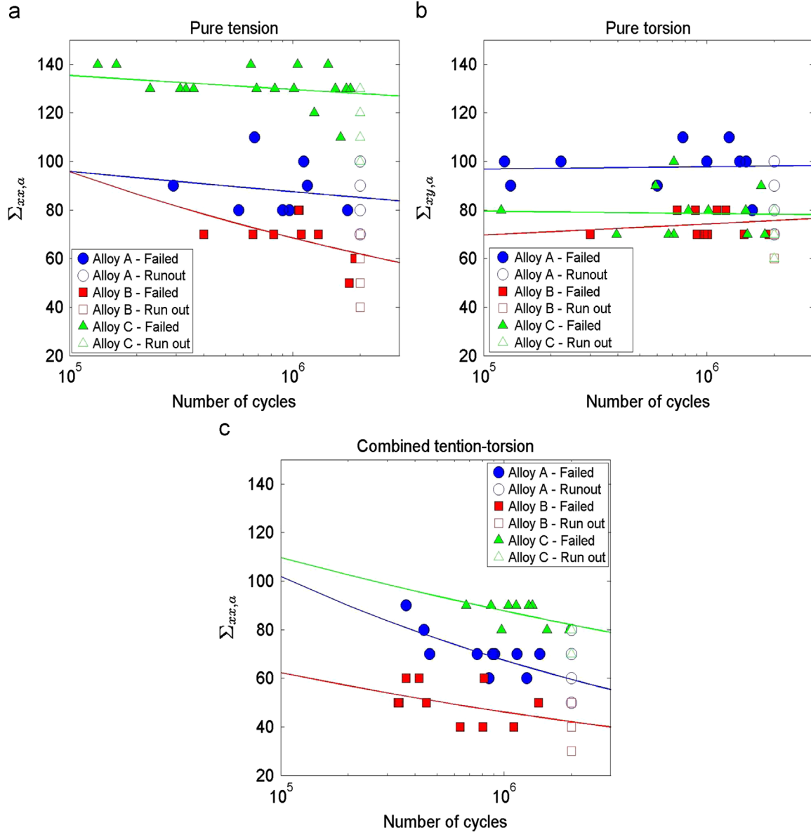
Fig. 8. Wöhler diagrams for alloys A, B and C for (a) uniaxial tensile loads R = -1 ; (b) reversed torsion load R = -1 (b); (c) combined tension-torsion load R = -1 .
