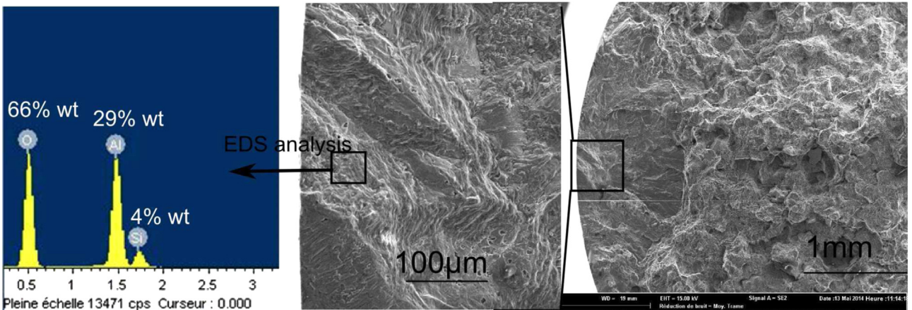
Fig. 13. Crack initiation due to the presence of an oxide film in pure tension loads. The local chemical composition and SEM observations of the failure surface for a specimen of alloy C.
