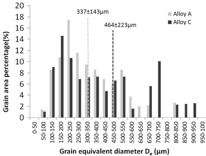
Fig. 5. Grain size considering the grain size percentage distributions of alloys A and C.
