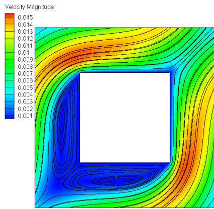
(a) Steady flow. Re_d = 29.1 ( Re^* = 12000 ).
