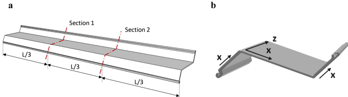
Fig. 3. (a) Localisation of the measures: XRD and ring core method in Section 1 and sectioning method in Section 2 ( L=6000 \text{ mm} ), (b) global reference frame.
