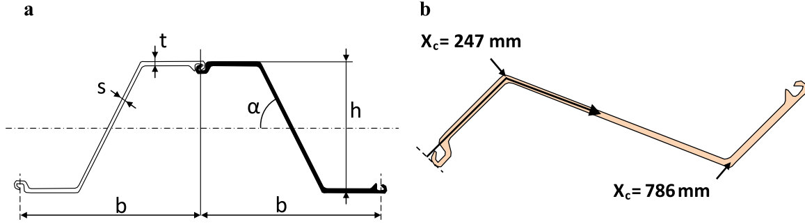
Fig. 2. (a) Sheet pile geometry (AZ 38-700+1, b=700 \text{ mm} , h=501 \text{ mm} , t=19 \text{ mm} , s=14.2 \text{ mm} , \alpha=63.2^\circ , length=6000 mm), (b) location of curvilinear coordinates: X_c .
