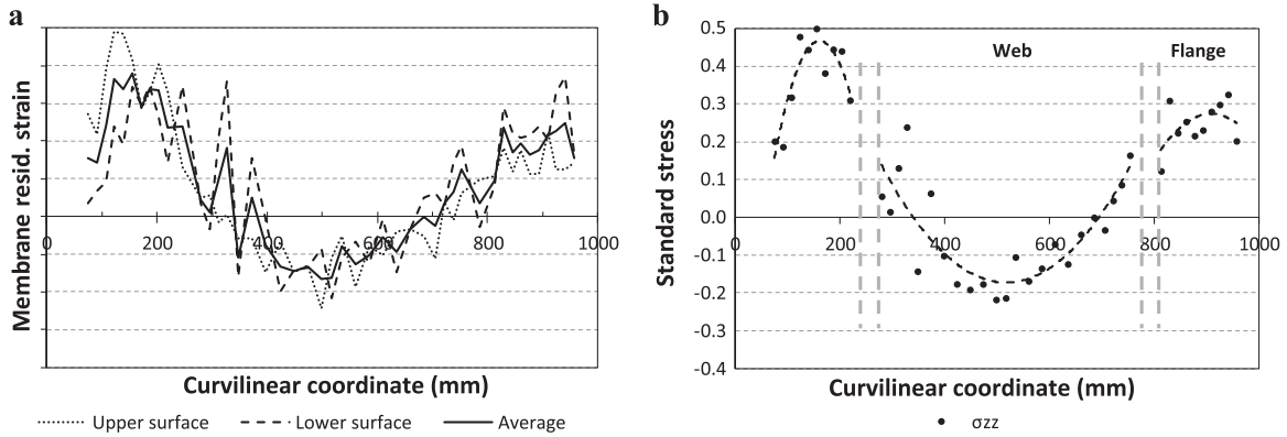
Fig. 13. (a) Membrane strain on the two surfaces & average strain in the sheet pile 2: after cooling, in the longitudinal direction, (b) normalised longitudinal residual stress in the sheet pile 2: after cooling, in the longitudinal direction.
