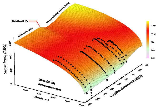
Figure 2. Comparison between experiments and analytical predictions for wide ranges of strain rates
