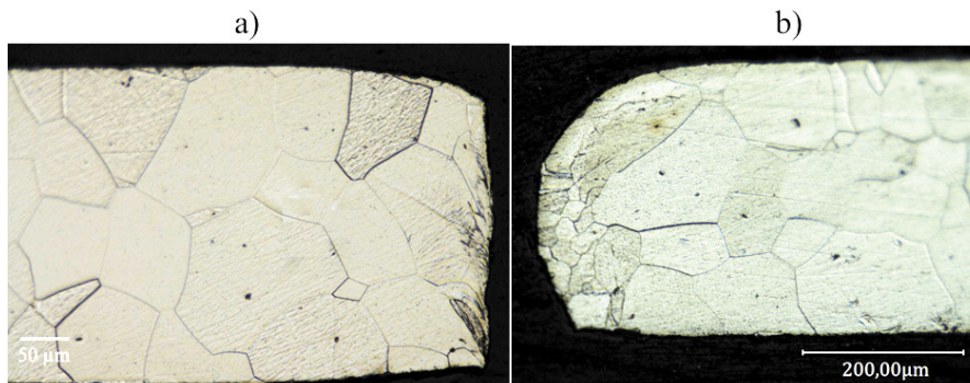
Fig. 2. (a) Punched edge with large grains and hardening (b) punched edge after annealing with local recrystallization
