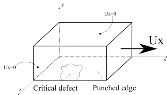
Fig. 8. Boundary conditions used for the FE simulations
