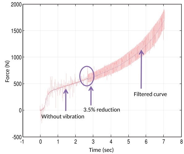
Fig. 14. Force versus time for a upset forging of plasticine in presence of sinusoidal vibration ( v_0 = 2.5 \text{ mm s}^{-1} , f = 45 \text{ Hz} and a = 18 \mu\text{m} ).
