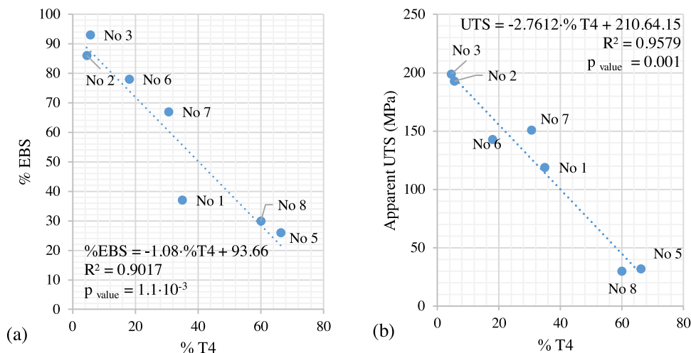
Fig. 15. Linear regression between% of T40/MZ interface occupied by morphology of type 4(%T4) and% of efficiently brazed T40/MZ surface (%EBS) obtained from fractography data (a); linear regression between% of T40/MZ interface occupied by morphology of type 4(%T4) and apparent UTS (b).
