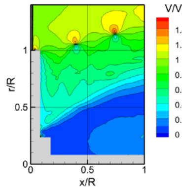
Fig. 8. b: Average velocity (experimental result) at TSR 5.06.
