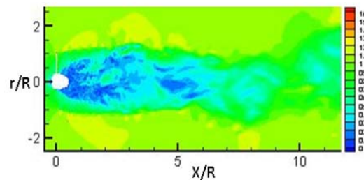
Fig. 10. c: velocity field at TSR 5.06.
