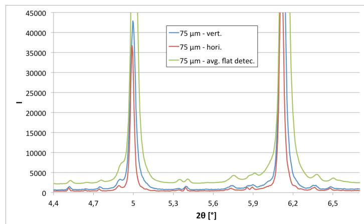
Figure 2: Horizontal and vertical diffraction analyses of a nitride Fe-3wt.%Cr-0.35wt.%C steel grade at a depth of 75 μm below the free surface. Use of a point detector and an analyser crystal in case of the horizontal scan. The averaging of the rings intensity from the flat detector analysis at the corresponding depth is given for comparison.
