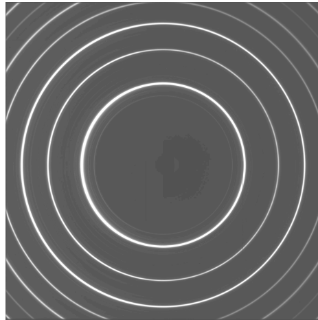
Figure 1: Scattering data imaging from high-energy synchrotron diffraction of a nitride Fe-3wt.%Cr-0.35wt.%C steel grade at a depth of 75 μm below the free surface. Main rings correspond to the scattering of the ferritic matrix.
