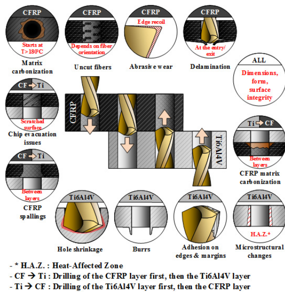
Fig. 1. Overview of the issues concerning Ti6Al4V/CFRP hybrid stacks drilling.
