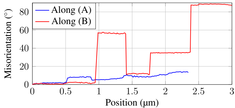
(c) Cumulative misorientation along (A) et (B) on the 64%-flowformed tube
