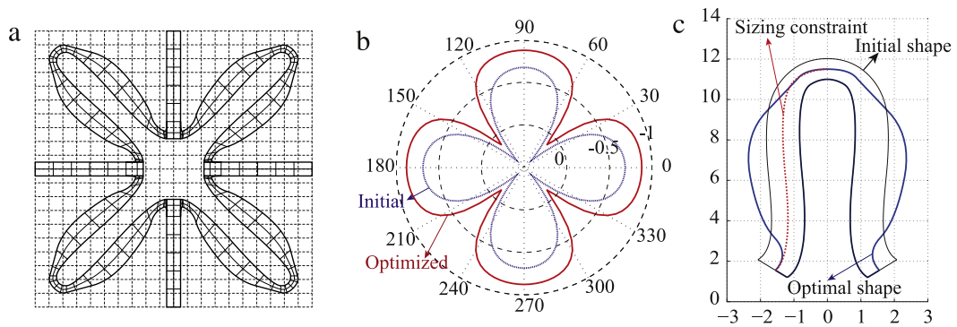
Fig. 13. Case 1: (a) full model of the optimized design. (b) Polar plot of the effective Poisson ratio for the optimized design. (c) Comparison between the size bounding polynomials, the initial and optimized designs.
