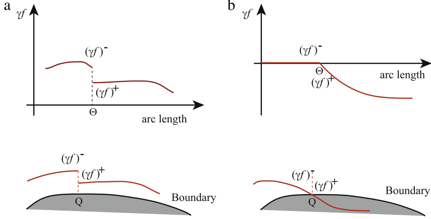
Fig. 11. Schematics of a 2D boundary integrand involving discontinuities.
