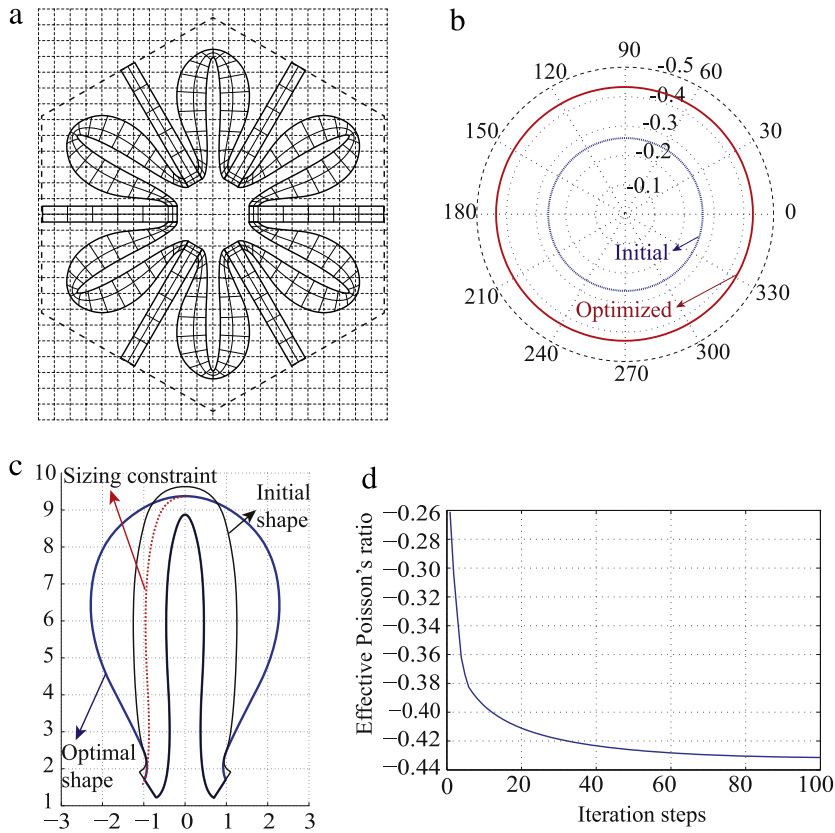
Fig. 19. (a) Full model of the optimized design. (b) Polar plot of the effective Poisson's ratio for the optimized design. (c) Comparison between the size bounding polynomials, the initial and optimized designs. (d) Iteration history of the objective function.
