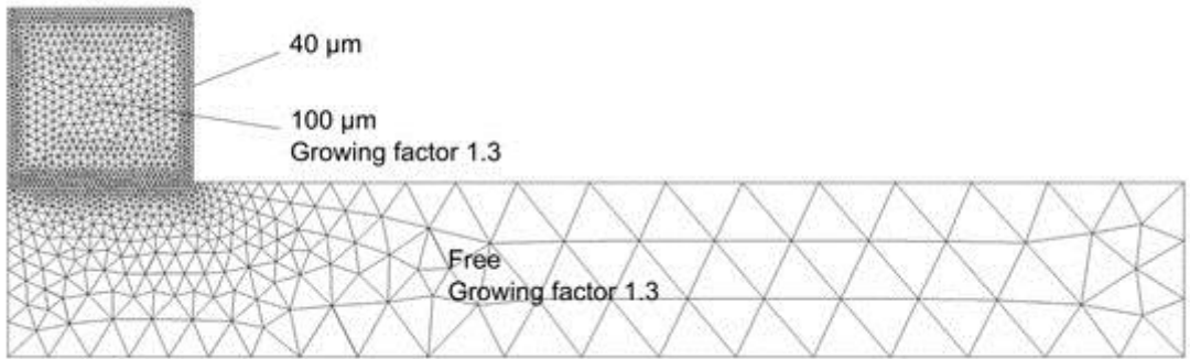
Figure 6. Mesh configuration.
