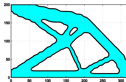
Figure 4: Optimised structure at the end of the NURBS-based TO method
