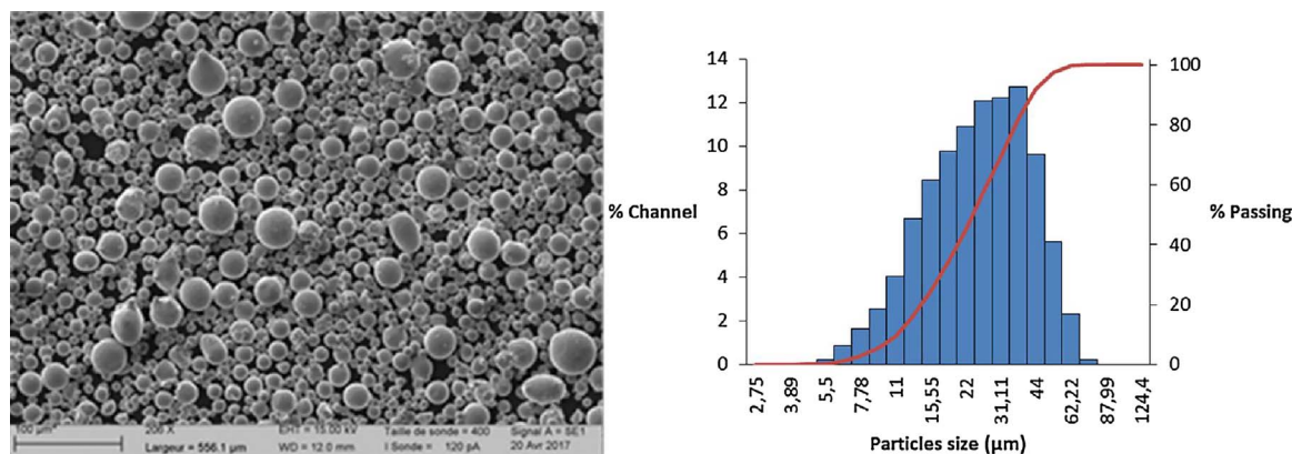
Fig. 1. (a) SEM analysis of powder particles, (b) Inconel 625 Grain distribution.
