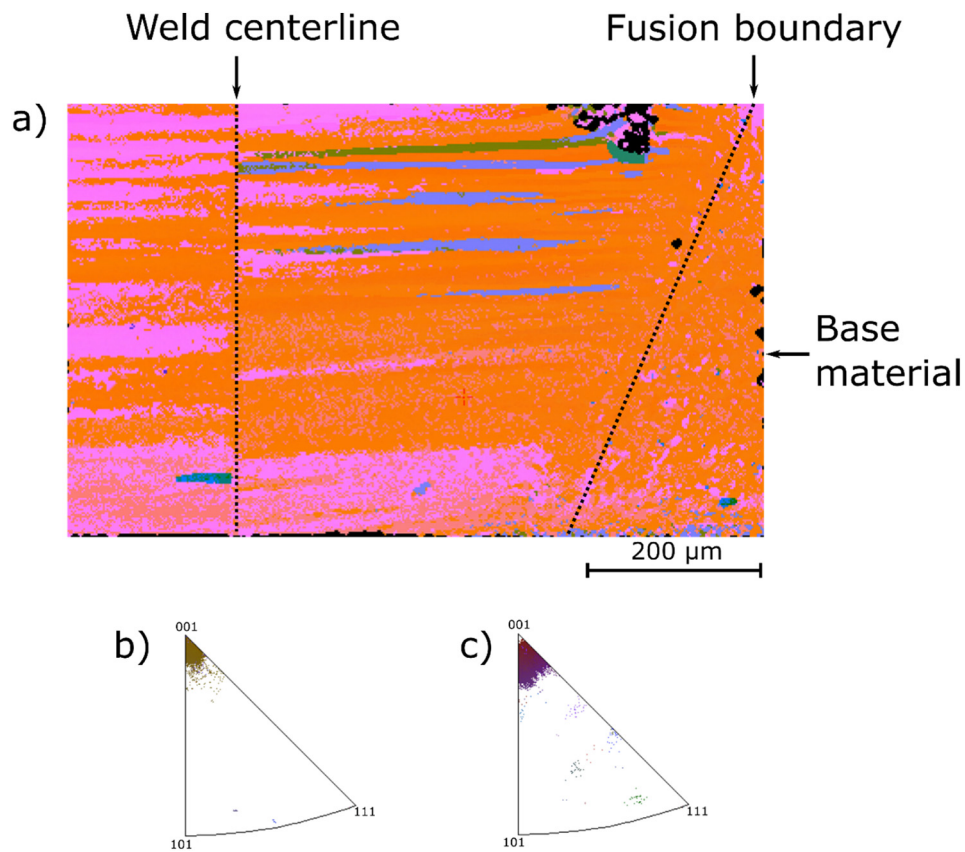
Fig. 3. a) Orientation map determined by EBSD; inverse pole figure in the tensile direction (wire axis) for the initial wire (b) and welded zone (c).
