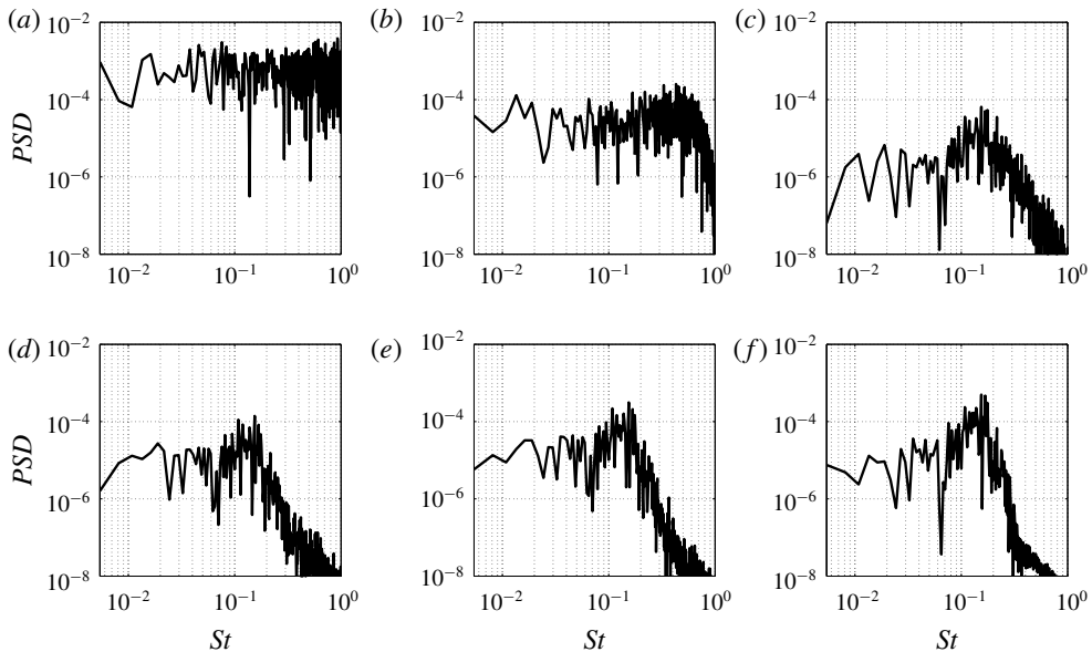
FIGURE 21. Fourier analysis performed on the time histories recorded on the monitoring probes (probe 1 – a; probe 2 – b; probe 3 – c; probe 4 – d; probe 5 – e; probe 6 – f). Power spectral density as a function of the Strouhal number.
