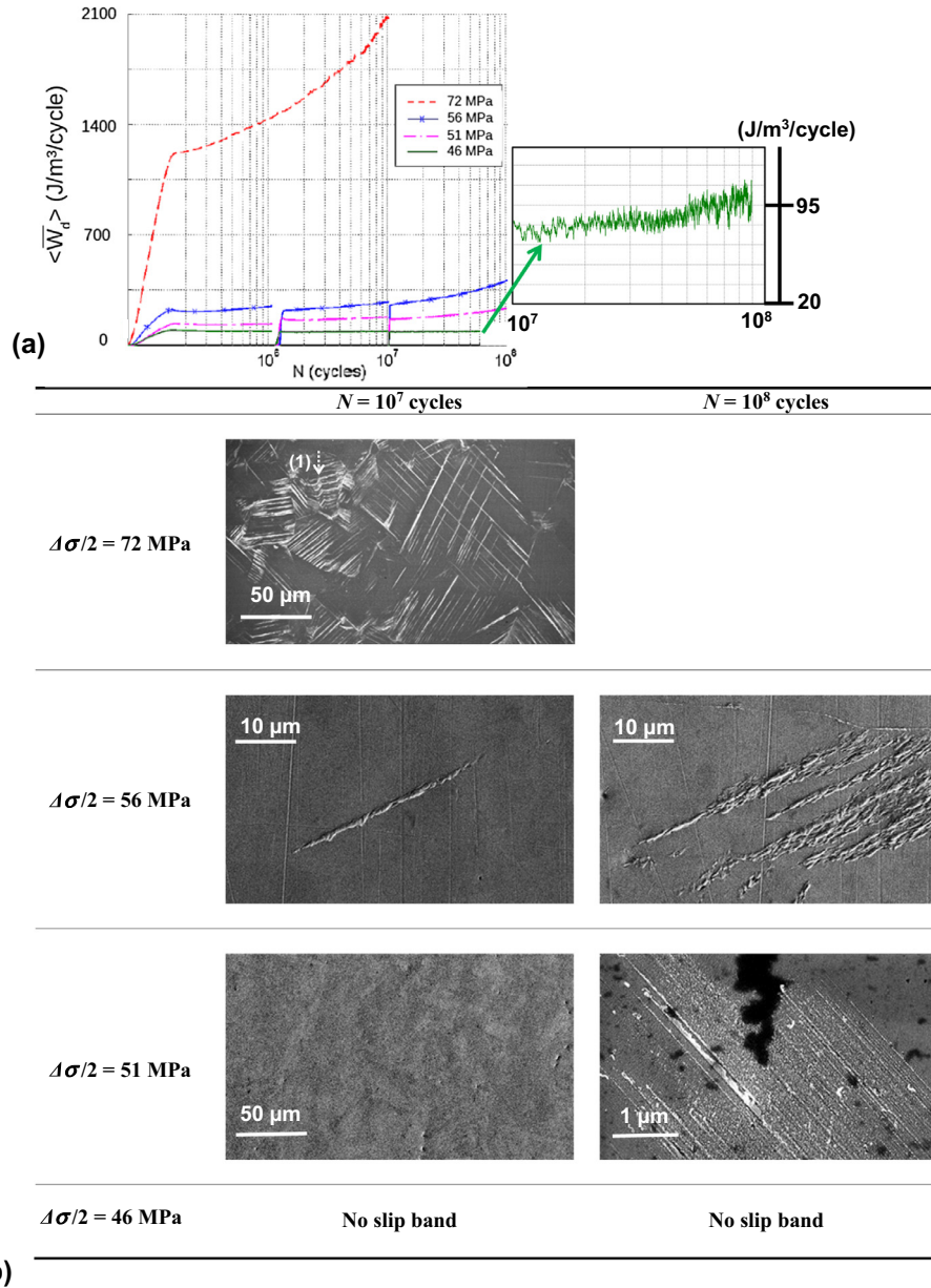
Fig. 11. Evolution of the mean dissipated energy \langle \overline{W}_d \rangle in fatigued copper as a function of the number of cycles (logarithmic scale). No cooling system was used: (a) evolution for various stress amplitudes, with zoomed example of recording at 46 MPa. (b) Scanning electron micrographs of the surface of the specimens after interruption of the fatigue tests after 10 7 and 10 8 cycles. The loading axis is horizontal. The white dotted line arrow on the micrograph corresponding to 72 MPa indicates slip bands transmitted through twin boundaries. The “(1)” indicates that the transmission occurred through two boundaries revealing the presence of a twin and two twin boundaries.
