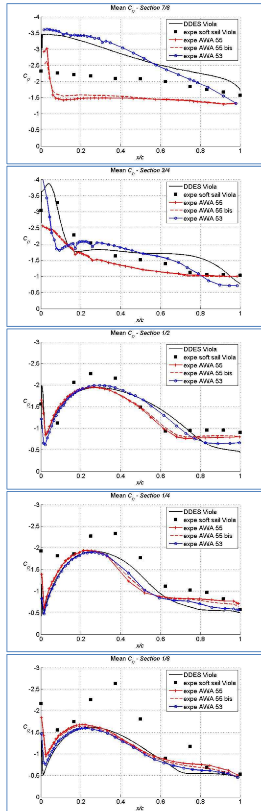
Figure 7: Cp measured on the solid spinnaker (present study) for AWA=53 and 55° (measurements from two distinct experimental runs are shown to assess the repeatability), measured on a soft sail [12] and computed with DDES [16].
