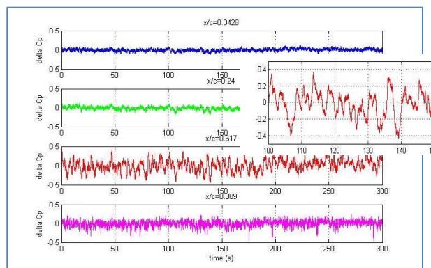
Figure 8: Time series of the C_p variations on section 1/2, at x/c=0.0428 , 0.240 , 0.617 and 0.889 , enlargement: detail for x/c=0.617 and t from 100 to 150s.
