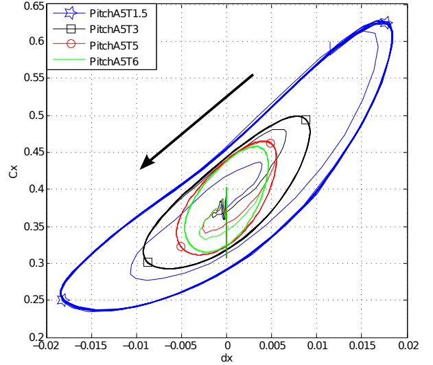
Figure 6: Driving force coefficient vs. non-dimensional displacement dx for pitching periods T=1.5, 3, 5 and 6 s. The loop area represents the work exchanged W .
