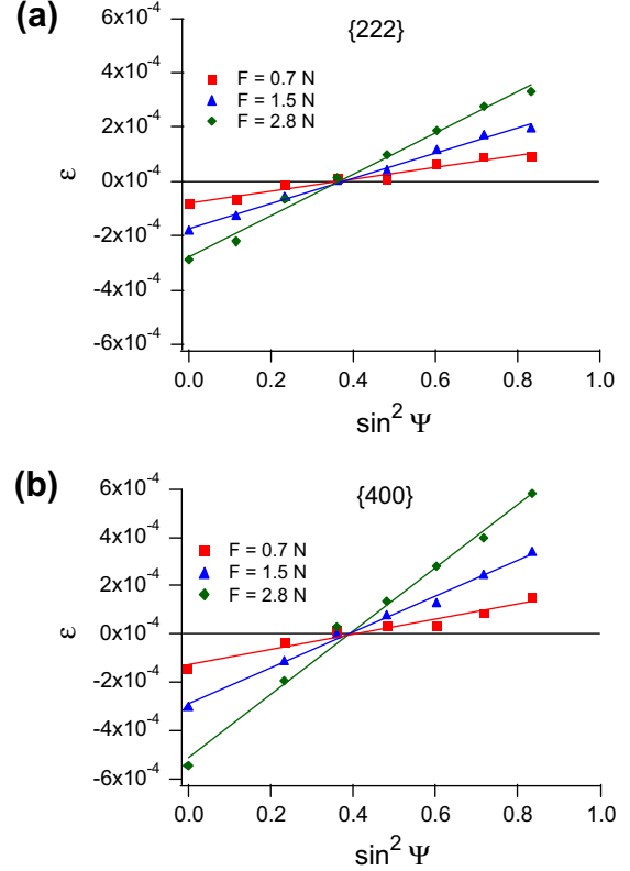
Fig. 4. Experimental X-ray lattice strains for (a) \{2\ 2\ 2\} and (b) \{4\ 0\ 0\} plane families as a function of \sin^2 \Psi , for the non-textured gold film.
