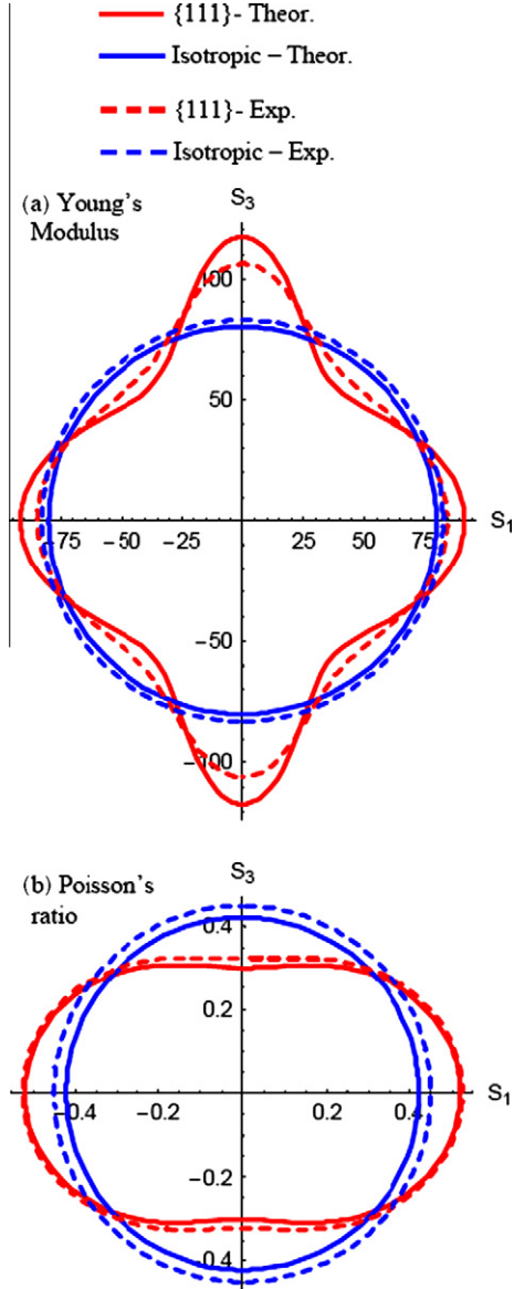
Fig. 10. Two-dimensional parametric surfaces of experimental and theoretical (a) Young's modulus and (b) Poisson's ratio, of perfect \{111\} -fiber-textured and non-textured gold films.
