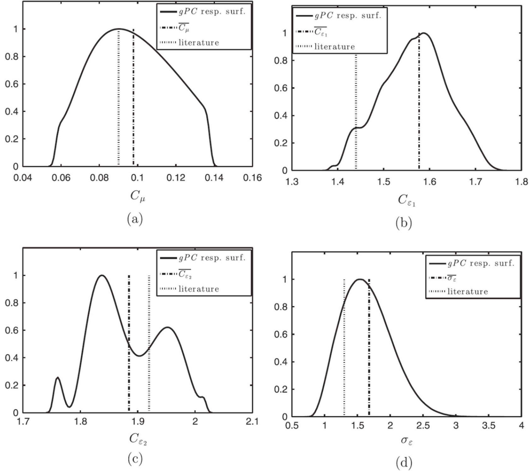
Fig. 10. Normalized probability density function (pdf/max(pdf)) of the Laufer–Sharma k - \epsilon model coefficients recovered through gPC. Figures reproduced with permission from Turgeon et al. [51].
