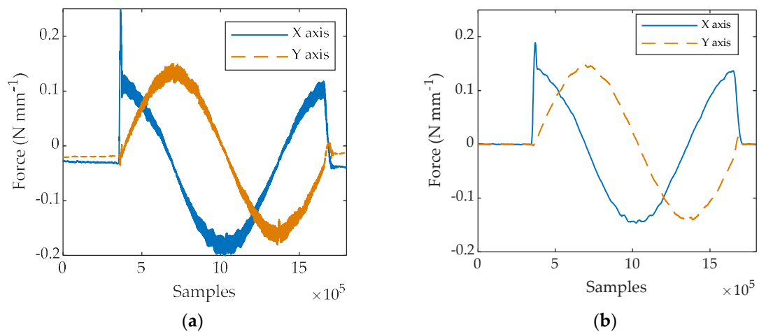
Figure 5. PTFE-machined up-milling with a depth of cut of 1.5 mm forces signals: (a) after applying a moving average on 10 cutting periods; (b) after applying a moving average on 10 cutting periods and a smoothing on 20 cutting periods. The signals after smoothing were also detrended.
