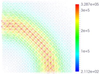
Fig. 10. Distribution of the eddy current density ( A/m^2 ) in a conducting plate.
