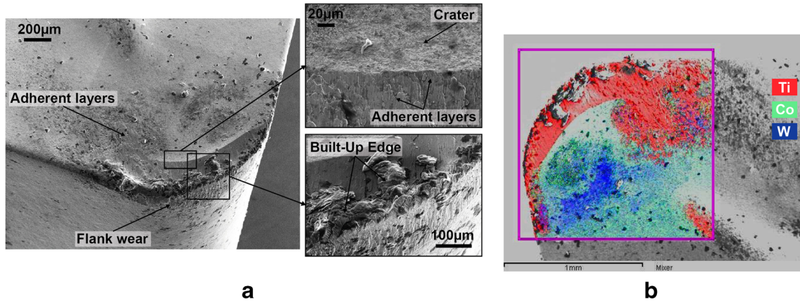
Fig. 5 Tool wear analysis (dry machining; T = 2.5 min; VB = 0.31 mm). a SEM analysis. b EDS analysis
