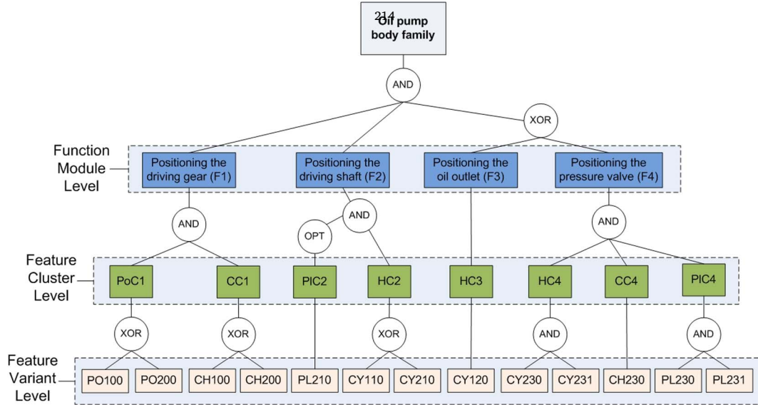
Fig. 12. Variety decomposition network for the oil pump body family.
