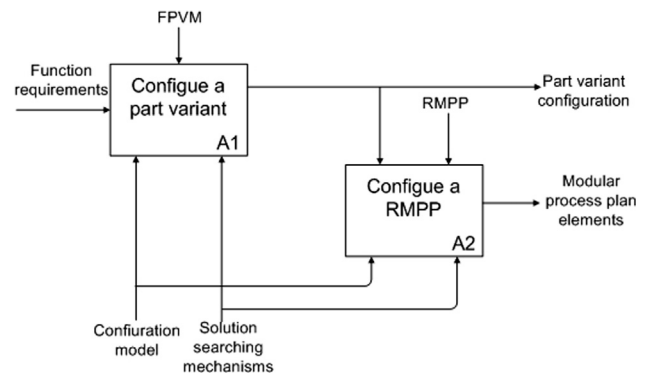
Fig. 9. IDEF0 diagram for integrated part configuration and RMPP configuration.
