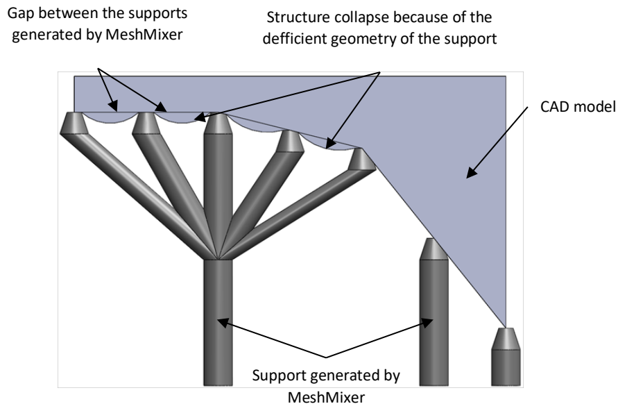
Example of a part and its support generated by MeshMixer
