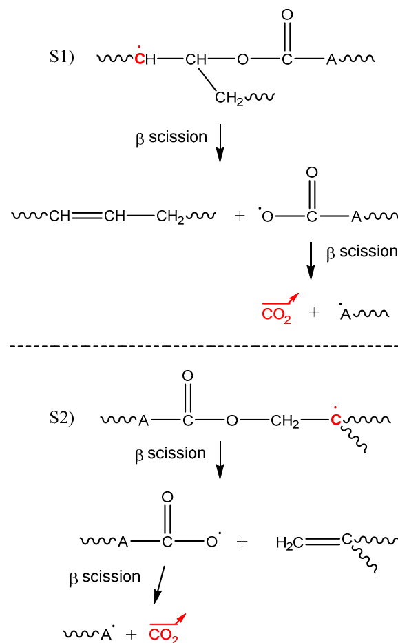
Scheme 5. Generation of volatile fragments (carbon dioxide) during the rearrangement of alkyl radicals.
