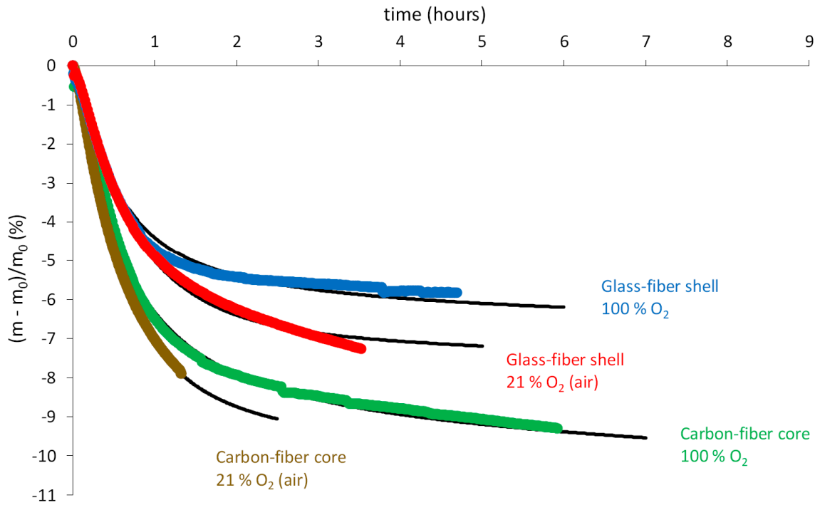
Figure 14 Mass changes of powder samples of carbon-fiber core in nitrogen between 180 and 210 °C (a) and of carbon-fiber core and glass-fiber shell in air and pure oxygen at 180 °C (b) and 210 °C (c): Comparison between simulations (black lines) and experimental data (color symbols).
