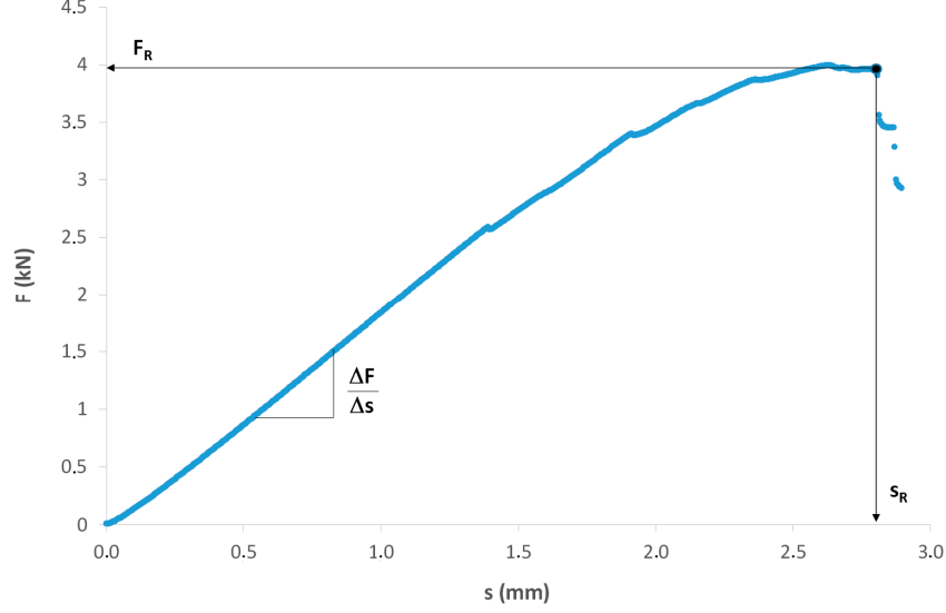
Figure 3. Example of load-displacement curve for the virgin composite rod.
