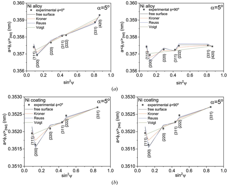
Figure 5 Examples of \langle a(\phi, \psi) \rangle_{\{hkl\}} versus \sin^2 \psi plots for the incident angle \alpha = 5^\circ , compared for different grain interaction models. The results for the ground sample (a) and electrodeposited layer (b) are shown. Error bars correspond to \delta(2\theta_{\{hkl\}}) = 0.01^\circ .
