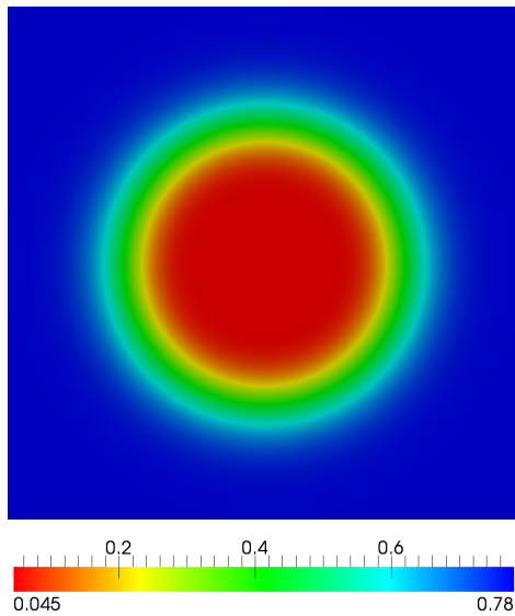
Figure 10: steady state of a single bubble immersed in liquid: Density field. For this simulation we use 64^2 elements and \Delta t = 10^{-4} . The EOS employed is the one plotted in figure 6.
