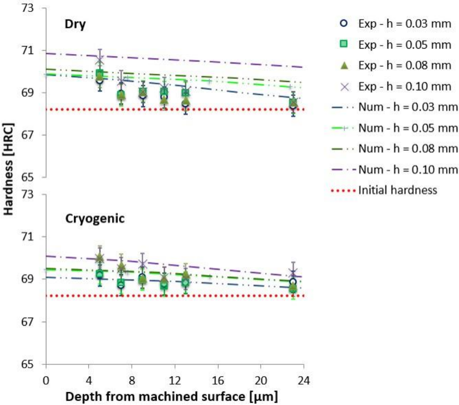
Figure11. Comparison between measured and predicted hardness for dry and cryogenic cooling.
