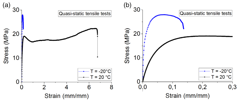
Figure 13. Figure 13 Tensile response of HDPE samples at 20 and -20^{\circ}\text{C} . [Color figure can be viewed at wileyonlinelibrary.com]
