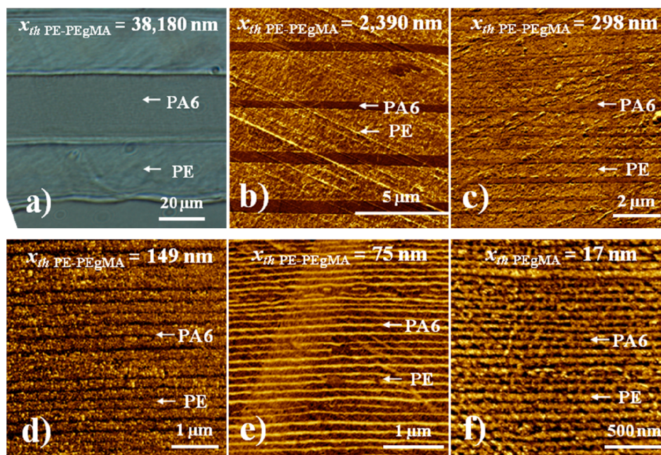
Figure 1. Optical (a) and AFM (b–f) images of PE/PEgMA/PA6 multilayer films
