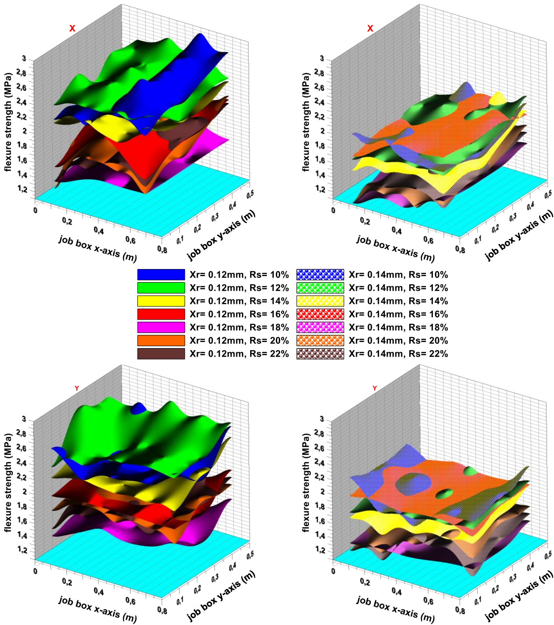
Fig. 5: Flexure strength ( \pm 0.05\text{MPa} ) as a function of job-box coordinate and process parameters (the actual points are connected to create these plot surfaces); for recoater speed between 10% and 22 %, (left, solid colour) X_r = 0.12\text{ mm} (right, dot-dot colour) X_r = 0.14\text{ mm} , and for (top) X and (bottom) Y orientation as indicated. (middle) This standard color code has been used in all of the following figures as well.
