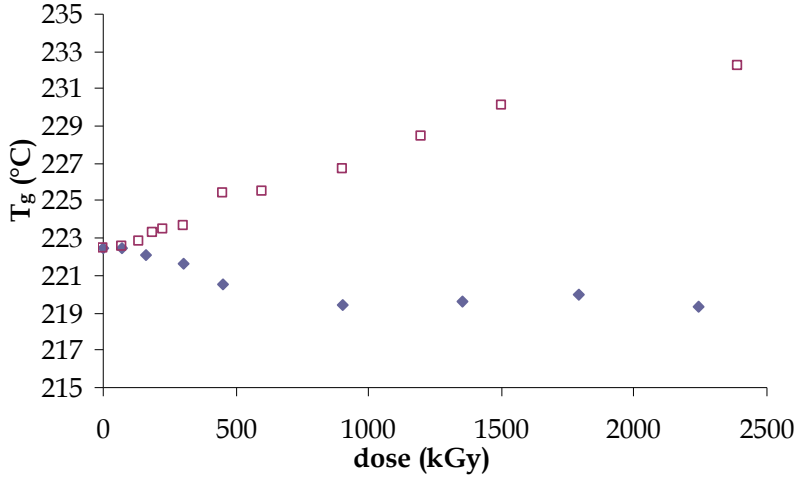
Fig. 6. Change in T_g for PES submitted to electron beam irradiation at room temperature ( \blacklozenge ) or 230°C ( \square ) (Li et al., 2006).
