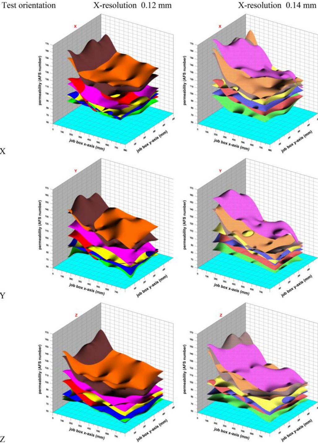
Figure A1 Permeability of the 3D printed specimen as a function of job-box coordinate and process parameters; for re-coater speed between 10 and 22%, (left) X_r = 0.12 mm (right) X_r = 0.14 mm and for X, Y, and Z orientation as indicated. See colour code in Figure A2 (Sivarupan et al., 2017)
