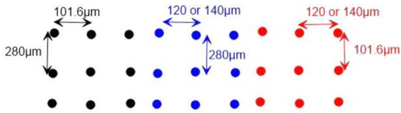
Figure 8 The special distribution of furan droplets perpendicular to X, Y, and Z directions, (the YZ, XZ, and XY planes, respectively)
